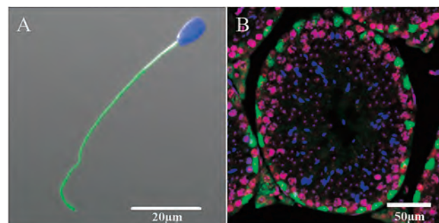
A. ウシ精子におけるCatSper1の発現(緑) B. マウス精細管横断面におけるSOX9の発現(緑) A. Localization of CatSper1 in bovine sperm (green). B. SOX9 expression of mouse seminiferous tubule cross-section (green).
